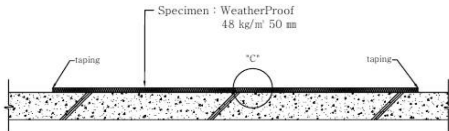
B-B' SECTION
