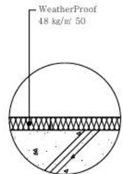
"C" Detail
