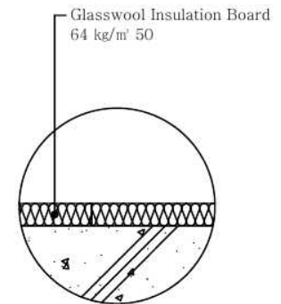
"C" Detail
