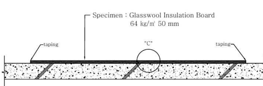
B-B' SECTION
