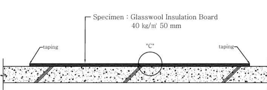
B-B' SECTION
