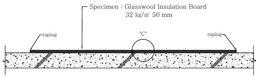
B-B' SECTION
