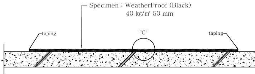
B-B' SECTION
