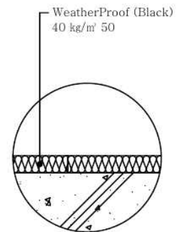
"C" Detail
