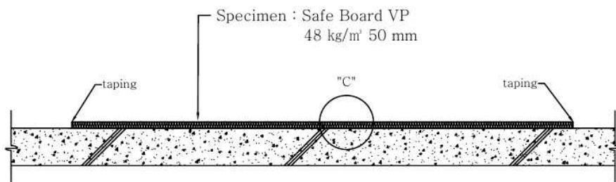
B-B' SECTION
