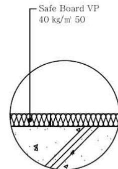
"C" Detail
