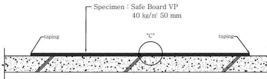
B-B' SECTION
