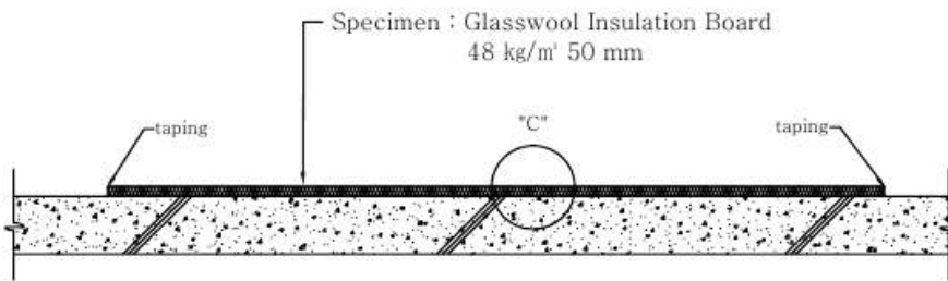
B-B' SECTION
