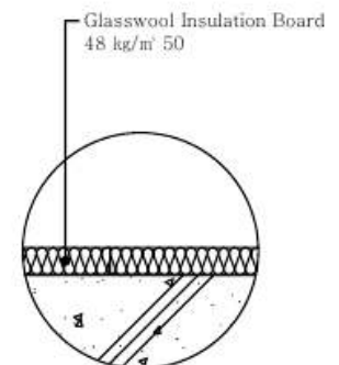
"C" Detail
