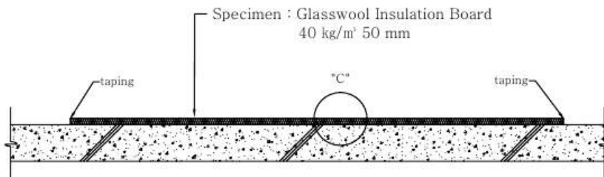
B-B' SECTION
