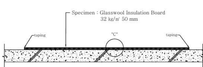
B-B' SECTION
