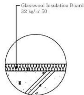
"C" Detail
