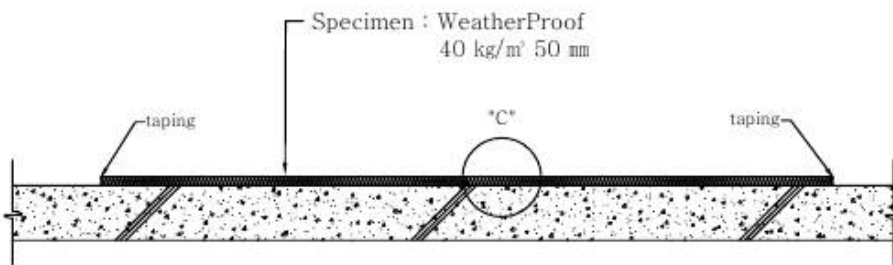
B-B' SECTION
